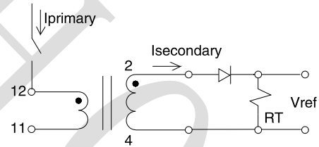
APPLICATION CIRCUIT
