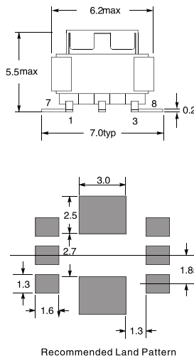
Recommended Land Pattern
